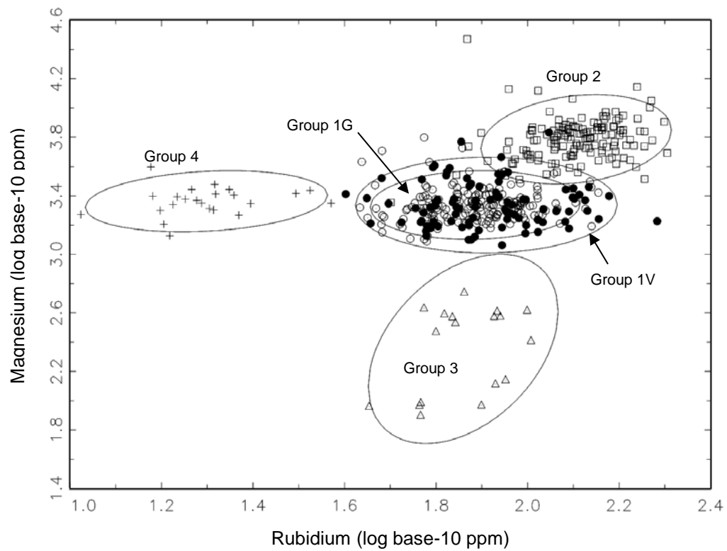
Figure 5.15. Bivariate plot of rubidium and magnesium showing five compositional groups in olivine-tempered ceramics.
