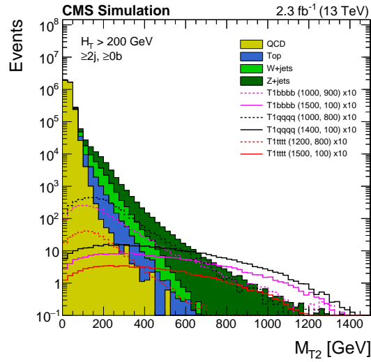
Figure 3.2: Inclusive distribution of M_{T2} . The SM backgrounds are stacked and example signal points are overlaid with their cross sections scaled up by a factor of 10. The signal models are described in Chapter 8. Only events with at least two jets are selected.
