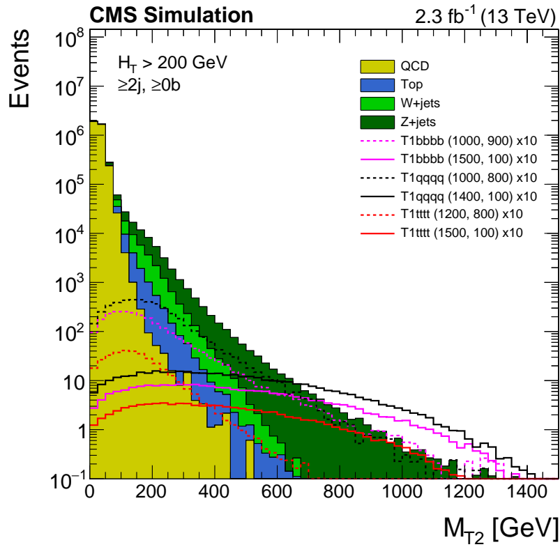
Figure 2.3: Inclusive distribution of M_{T2} after the baseline analysis selection. The SM backgrounds are stacked and example signal points are overlaid with their cross sections scaled up by a factor of 10. Only events with at least two jets are selected. T1bbbb, T1qqqq, and T1tttt represent possible SUSY signal models to be further discussed in chapter 8.
