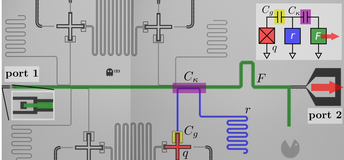
Figure 4.6: Micrograph of the device. The false color corresponds to the colors used in the lumped element model, shown in the top right inset. Signals enter the system through a feed line at port 1. The filter F is formed by a standing wave resonator embedded into the feed line. The feed line is interrupted by a capacitance (left inset) at one end and shorted to ground on the other, forming a \lambda/4 resonance. Signals injected at port 1 are mostly reflected by the weak input capacitance. The transmitted energy rings up the filter resonance. Energy leaves the filter through a tap near the shorted end at port 2. The red arrow indicates the path by which energy leaves the filter through a wire bond (not shown) and enters the external detection hardware, including a parametric and HEMT amplifier. The measurement resonators r are connected to the filter via capacitance C_\kappa formed by the proximity of the filter and resonator traces. The resonator couples to the qubit q through an inter-digitated capacitor C_g . Note that the design allows for an independent resonator for each qubit while allowing several resonators to share a single filter. Note also the filter requires near zero additional on-chip area.
