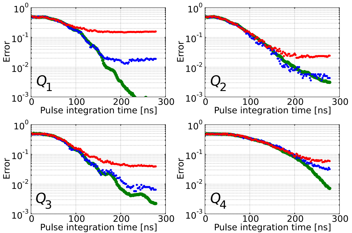
Figure 6.10: Simultaneous measurement of four qubits. Separation (green) and state (blue and red) fidelities are shown similarly to Fig. 6.9. Ripples on qubits Q_1 and Q_3 were caused by spectral leakage.
