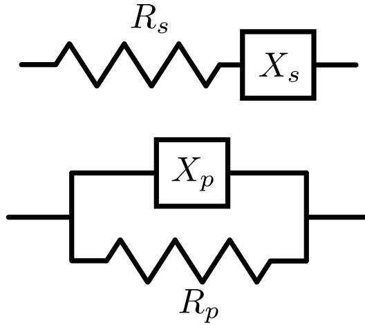
Figure F.1: Series and parallel circuits. The reactances X_S and X_P can be capacitive or inductive.
