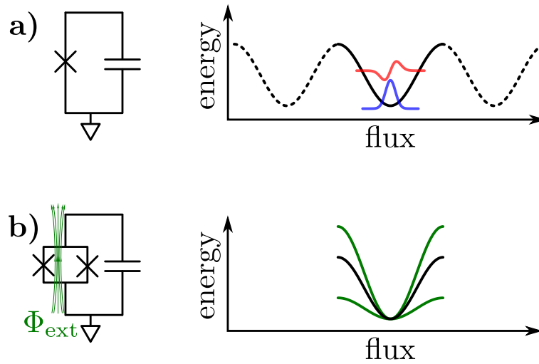
Figure 2.5: The transmon circuit and energy potential. a) The transmon is similar to a parallel LC oscillator, but with a nonlinear inductor. The potential energy has the shape of a cosine, and the large C , analogous to a large mass, prevents the wave functions from tunneling between wells. b) The single junction is replaced by a loop with a pair of junctions. External flux is used to modulate the effective critical current of the loop, which changes the height of the potential energy. This in turn causes the resonance frequency to shift.
