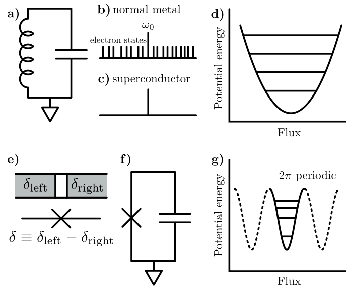
Figure 1.5: Superconducting qubits. a) A parallel LC circuit. b) The excitation spectrum of the system constructed with normal metal includes a dense set of electron excitations. These excitations interact with the circuit resonance and destroy quantum coherence. c) If the circuit is constructed with superconducting metal, the electron states vanish, leaving the circuit mode isolated and able to exhibit quantum coherence. d) The quantized mode of the LC circuit. The quadratic potential leads to equally spaced energy levels. e) A Josephson junction is formed by a thin insulating barrier interrupting two superconducting electrodes. The circuit model symbol for a Josephson junction is a cross. f) Replacing the linear inductor with a Josephson junction creates an anharmonic oscillator. g) The anharmonicity leads to unequally spaced energy levels. The lowest two levels can be used as a qubit.
