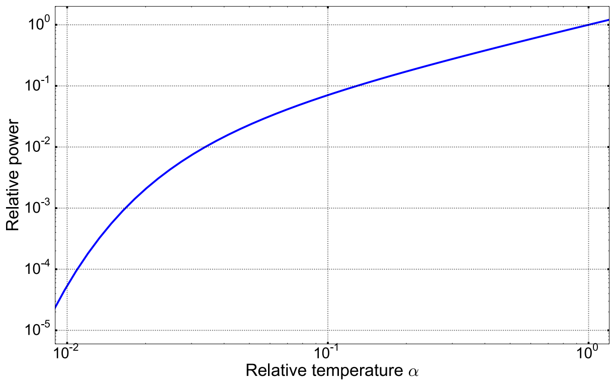
Figure 5.2: Ratio of voltage noise spectral density S_V(\alpha T)/S_V(T) for T = 4 K and f = 6 GHz.
