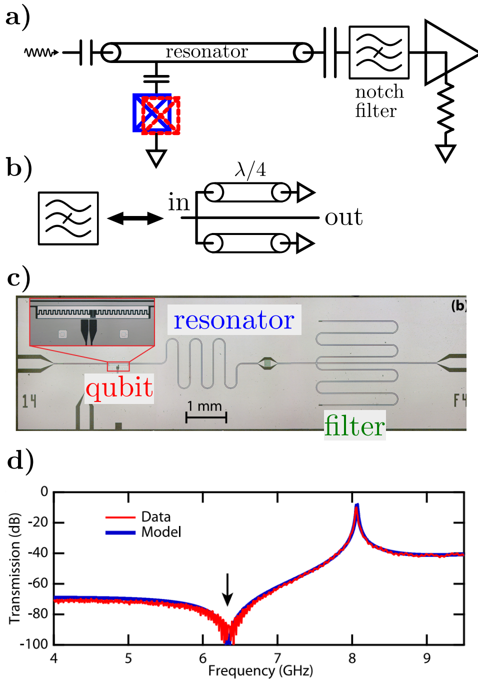
Figure 2.9: A filter used to increase the \kappa_r T_1 product. a) The filter is placed on the output of the resonator to prevent radiation at the qubit frequency from leaving the system. b) The filter was implemented as a symmetric pair of \lambda/4 stubs to ground. c) Micrograph of the Yale device. The filter is seen on the right side as two meandering co-planar waveguide resonators. d) Transmission through the system. Note the notch just above 6 GHz, which protects the qubit. The large increase in transmission at 8 GHz is the resonance frequency of the resonator.
