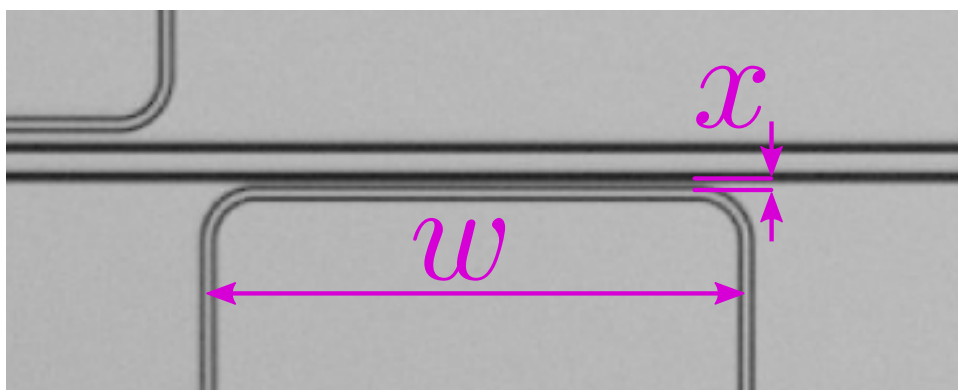
Figure 4.10: Coupling between a measurement resonator and the filter.
