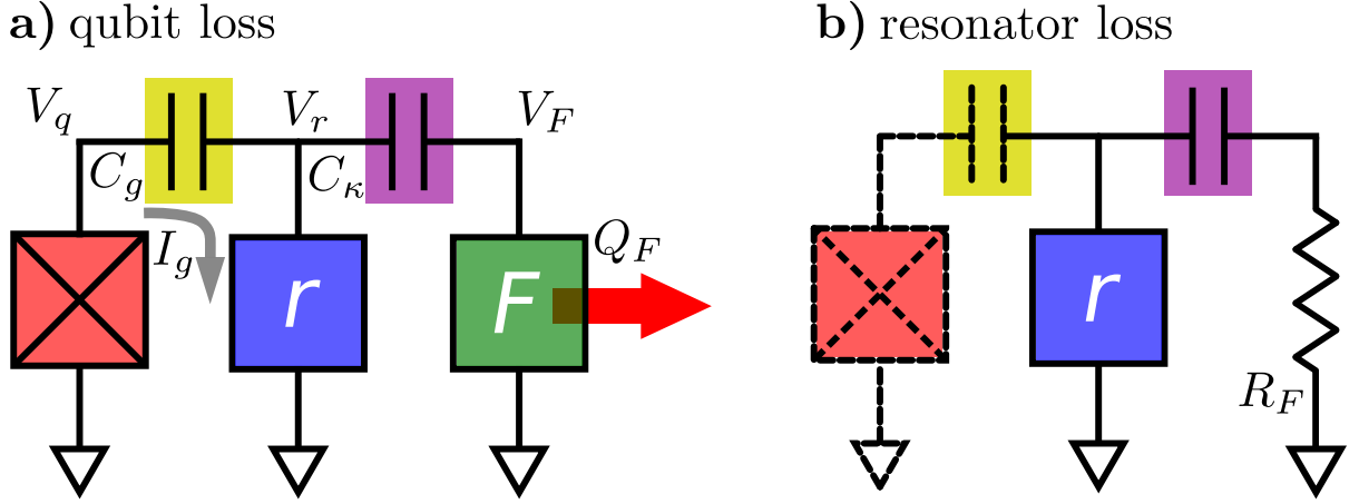
Figure 4.3: Lumped element model of the qubit and measurement circuit. a) The circuit is a ladder of alternating coupling capacitors and shunt resonators to ground. The only path by which energy can leave the system is through the finite internal quality factor Q_F of the filter, as indicated by the red arrow. At the qubit frequency, the impedance of the coupling capacitors is greater than the impedance of the resonators. This means that most of the current flowing through eg. C_g goes to ground through resonator r . b) To understand the quality factor of the resonator Q_r , we neglect the qubit which is assumed to be lossless. The damping of the resonator therefore comes entirely from the loss of the filter. Near resonance the filter impedance is a pure resistance.
