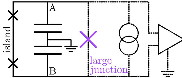
Figure 2.4: The quantronium qubit. The leftmost branch is essentially a charge qubit with two junctions connecting the island to the reservoir. The extra capacitance in the next branch reduces the quantronium’s sensitivity to charge noise. The rightmost three branches, shown in dotted line, are used for measurement. With the current source off, the circuit mode is symmetric from top to bottom and does not couple into the amplifier or large junction. Turning on the current bias breaks this symmetry, and when the large junction switches to the voltage state that voltage is measured by the amplifier.
