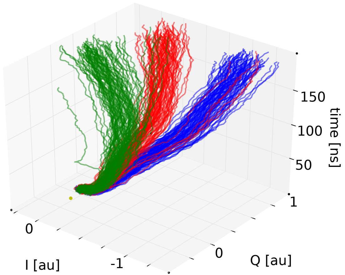
Figure 6.8: IQ trajectories during integration of the measurement pulse, showing approximately 150 separate measurements. The three branches correspond to the qubit prepared in the |0\rangle (blue), |1\rangle (red), or |2\rangle (green) states. Note the green threads which jump to the red branch part way through the measurement, which represent |2\rangle \rightarrow |1\rangle qubit transitions.
