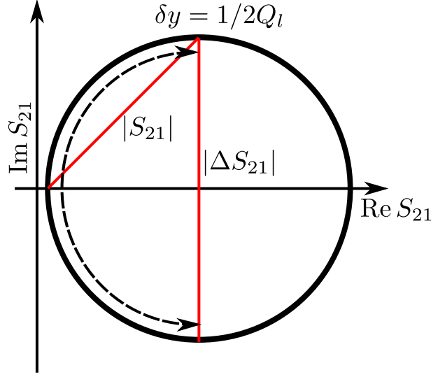
Figure 3.2: Scattering diagram for shunt resonator
