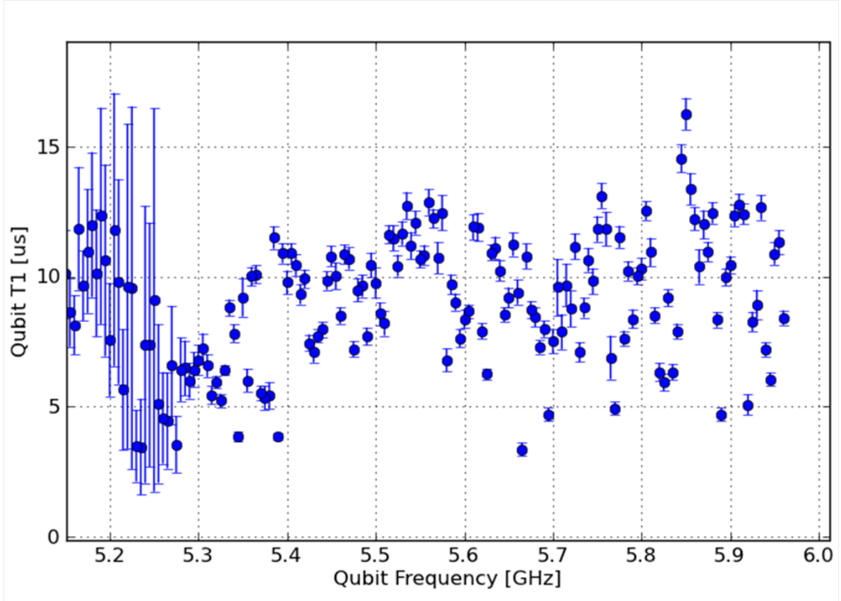
Figure 6.6: Energy decay time T_1 versus frequency for qubit Q_2 . With the measurement resonator frequency above the qubit, the lack of downward trend in T_1 with increasing qubit frequency indicates that the measurement circuit does not dominate the qubit damping. The T_1 values are distributed around 10 \mu\text{s} , which is several times larger than the Purcell limit predicted in the absence of the filter. The dip and wild variation in T_1 5.2 GHz come from coupling to a resonator bus which was not used in this experiment.
