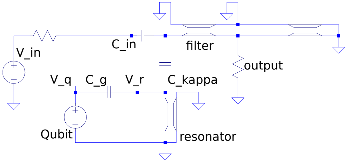
Figure 4.4: Screen capture of the SPICE model. The qubit is replaced by a voltage source which is activated with an ac signal of amplitude V_s at variable frequency \omega . The current I_s through the source is probed and the admittance of the external circuit computed as Y_e(\omega) = I_s/V_s . Note that the filter \lambda/4 transmission line resonator is not drawn to scale; the end which connects to ground is physically shorter than the other section.
