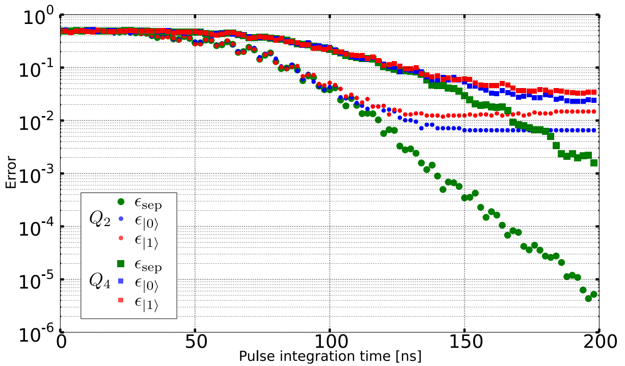
Figure 6.9: Time dependence of measurement errors for qubits Q_2 (circles) and qubit Q_4 (squares) measured simultaneously. Green points indicate the separation error \epsilon_{\text{sep}} , while the blue and red points represent \epsilon_{|0\rangle} and \epsilon_{|1\rangle} respectively. The data in Fig.6.7 came from the t = 140 ns point for Q_2 .
