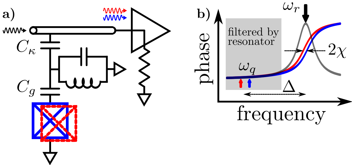
Figure 2.8: Schematic for measurement with an auxiliary resonator. a) The qubit is protected from resistance in the external circuitry by a detuned resonator which acts as a short at the qubit frequency. b) The qubit states cause the resonator frequency to shift, leading to large measurable phase shift at the resonator frequency.
