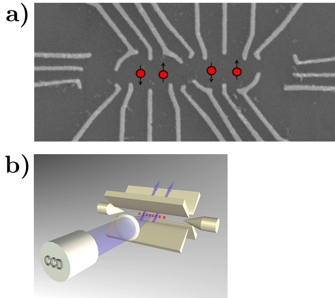
Figure 1.4: Qubit implementations. a) Electrons embedded in a semiconductor are used as qubits through their spin degree of freedom. This image shows a pair of “double quantum dot” qubits. In each one, two electrons are used to implement a single logical qubit. Note the large number of control wires. The image was taken from the website of Amir Yacoby at Harvard. b) Ions trapped in a linear “Paul trap”. Blue arrows indicate axes through which laser light is brought into the trap to control the qubit states. State measurement is done through a state dependent fluorescent technique and the outgoing light is collected by a CCD camera. The image was taken from the website of Rainer Blatt at Innsbruck.
