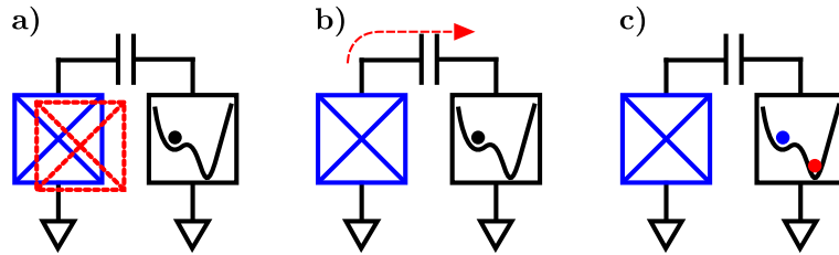
Figure 2.6: Qubit measurement by swapping the excitation into an auxiliary circuit. (a) The qubit starts in a superposition of the ground (blue) and excited (red) states. (b) The qubit is brought on resonance with the detector. If it was in the excited state, one quantum of energy is swapped into the detector, otherwise nothing happens. In either case, the qubit is left in the ground state. (c) The qubit is brought off resonance with the detector to turn the interaction off. The detector is now in one of two measurably different states corresponding to the two possible qubit states.
