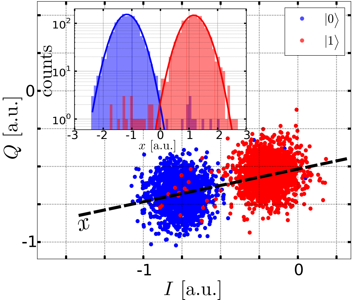
Figure 6.7: Measurement events for one qubit after 140 ns pulse integration. Points in the wrong cluster are due to unwanted qubit state transitions. The appearance of more red points in the blue cluster than blue points in the red cluster is partially an artefact of the plot, and partially due to the fact that the qubit undergoes more downward transitions than upward transitions. The inset shows histograms of the IQ points projected onto the line connecting the centers of the |0\rangle and |1\rangle clouds. Heavy lines are Gaussian fits to the histograms are used for computing the separation error.
