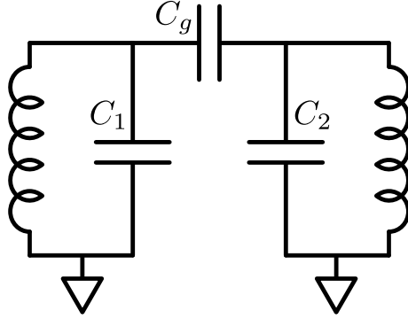
Figure D.2: Two circuits coupled through a capacitor C_g .
