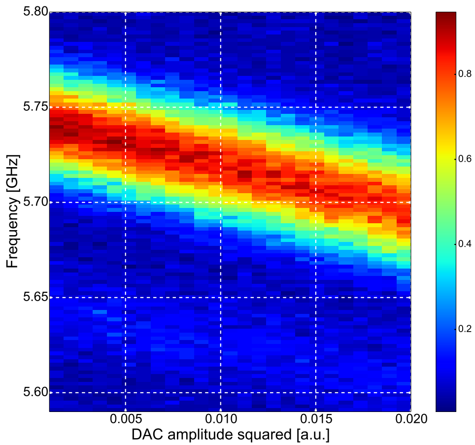
Figure 6.4: AC Stark shift measured via qubit detuning during measurement.
