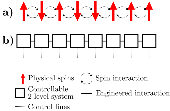
Figure 1.3: The physics of a quantum spin chain can be investigated by construction of a controllable and measurable analogue system. a) A physical spin chain. b) An array of two level systems engineered to match the physics of the spin chain.
