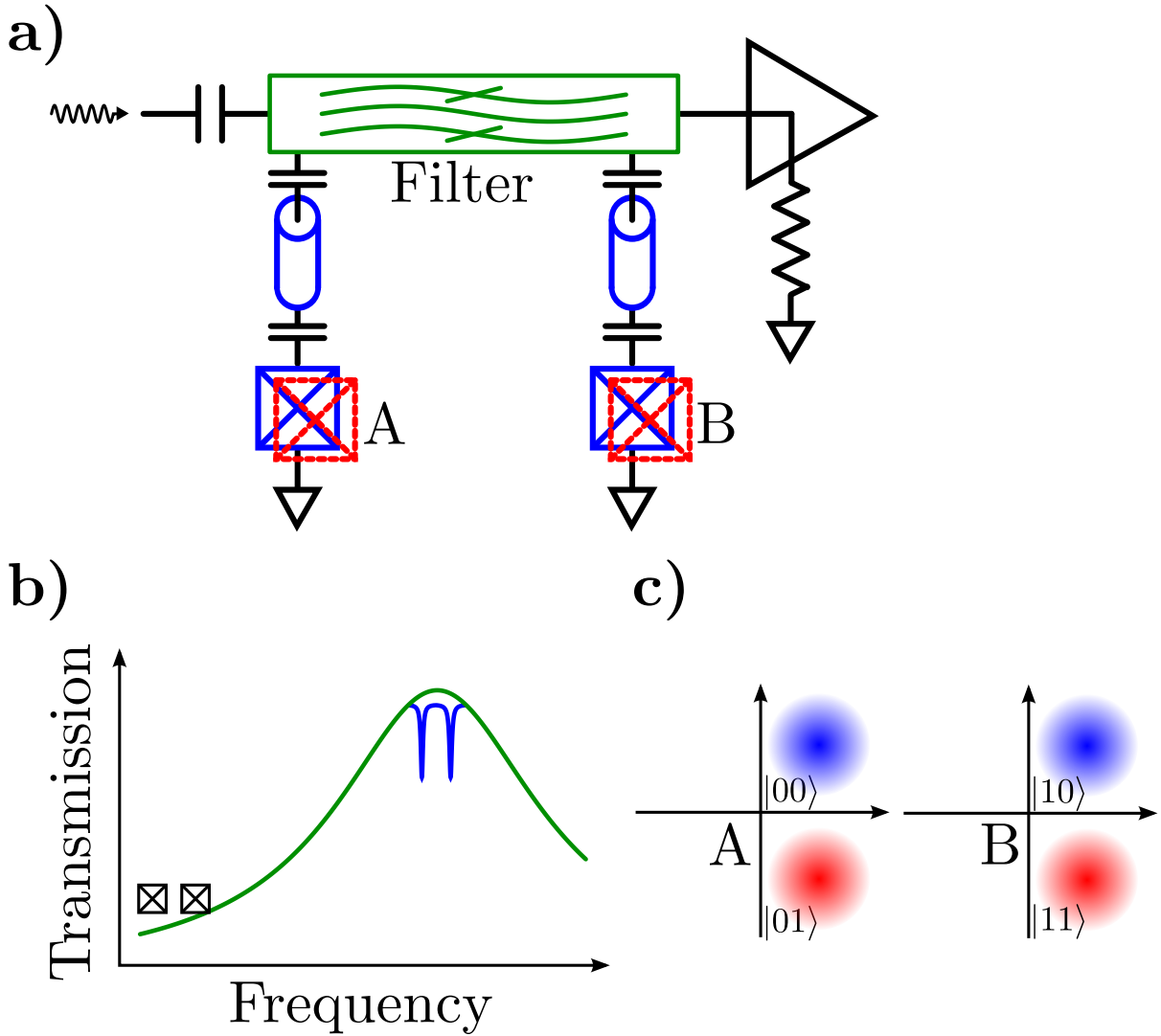
Figure 4.2: Bandpass filter circuit topology. a) Several measurement resonators (blue) connect in parallel to the microwave feed line, each one connected to a single qubit. The filter (green) is embedded directly into the feed line. b) The measurement resonators, which produce dips in the transmission spectrum, are all placed within the filter pass band. The qubits sit out of the pass band and are protected from emission. c) Each resonator's amplitude and phase contains the information of only one qubit state.
