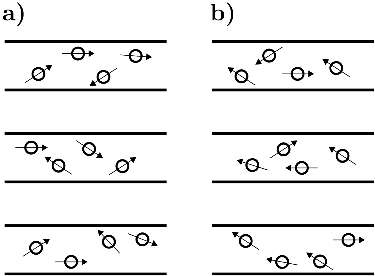
Figure 1.2: A wire with two different macroscopic current states.(a) and (b) show three microscopic states corresponding respectively to rightward and leftward current. Note that in each microscopic state some electrons may be moving in a direction against the macroscopic current.
