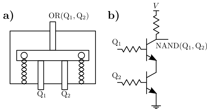
Figure 1.1: Two physical implementations of logic elements. a) A mechanical OR gate. If either of the bottom rods is pushed, the output rod extends. If neither input rod is pushed, springs retract the output rod. b) An electronic NAND gate. If voltage is applied to both input wires then current flows freely through the transistors, bringing the output node to ground.
