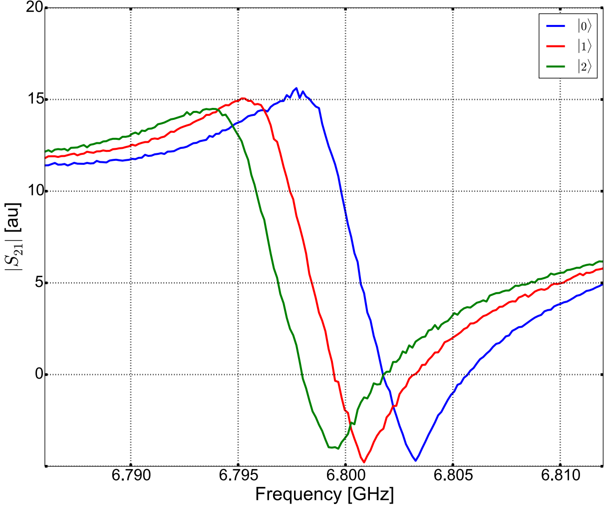
Figure 6.2: Transmission through the measurement circuit for three qubit states. Asymmetry in the resonance dips comes from impedance mismatch in the input and output of the measurement circuit.
