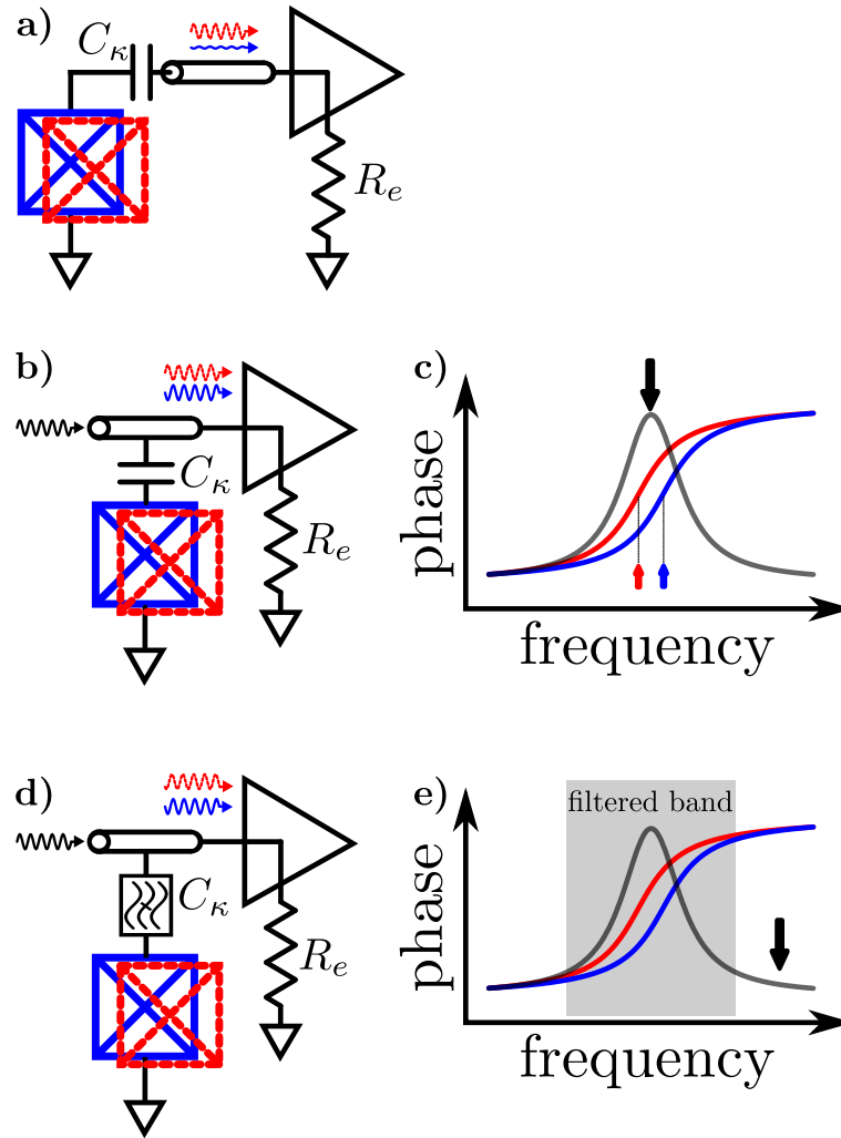
Figure 2.7: Measurement based on traveling waves. a) The qubit state is determined by the presence or absence of an outgoing wave. As the maximum measured energy is just the single photon in the qubit, the signal to noise ratio is too low. b,c) An externally supplied voltage is used to raise the signal to noise ratio. The wave acquires a qubit state dependent phase shift as it scatters from the shunt line containing the qubit. The blue and red curves indicate the phase response for the qubit in |0\rangle and |1\rangle , respectively. The gray curve indicates the difference in these phases. The center frequencies of the qubit in the ground and excited states are indicated by the blue and red arrows, and the frequency yielding the maximum phase signal is indicated by the black arrow. d,e) A filter placed between the qubit and external resistance could raise the limit on qubit lifetime, but this leads to a smaller detectable phase shift.
