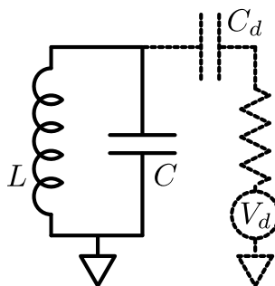
Figure D.1: A parallel LC circuit. The main circuit is shown in solid line, while the driving circuit is shown in dotted line.
