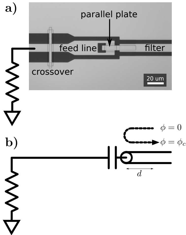
Figure 4.7: Input capacitor for the filter. a) Micrograph of the device. The feed line comes in from the left and the filter coplanar waveguide resonator is on the right. A thin film of \text{SiO}_2 separates the connecting aluminum strip on the feed line side. A hole in the feed line renders the overlap area insensitive to optical lithography misalignment. The connecting strip contacts the filter resonator directly. b) Circuit model. A wave reflecting from the input capacitor acquires a phase shift which effectively increases the length of the filter.
