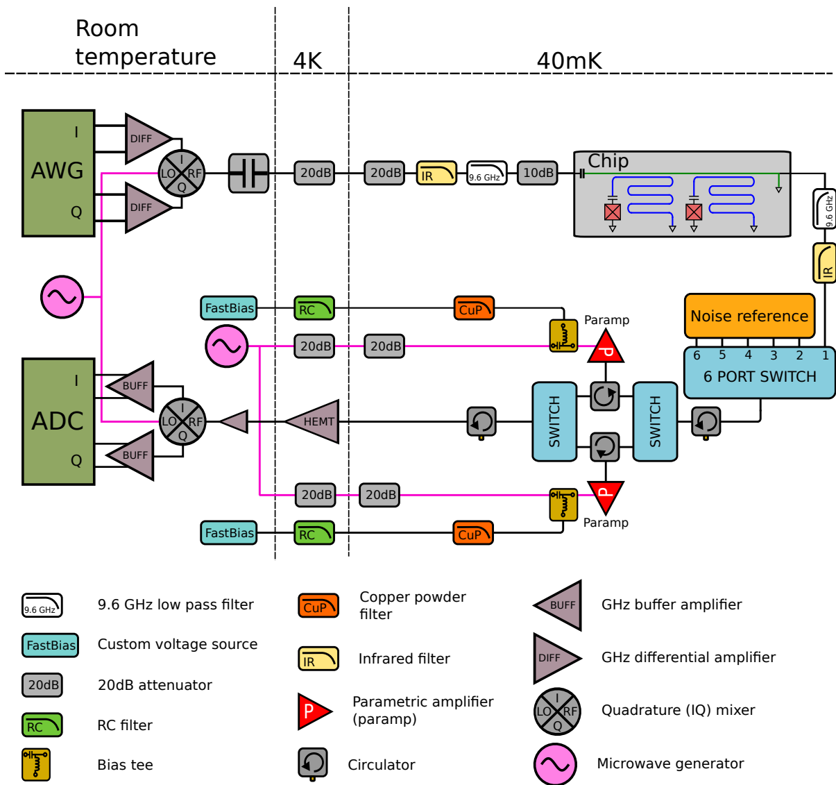
Figure 5.1: Schematic of the measurement system.
