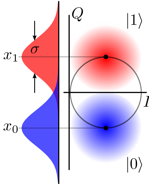
Figure 3.3: IQ clouds for the qubit states measured in the presence of noise. The clouds for |0\rangle (blue) and |1\rangle (red) are centered on the diametrically opposite points of the S_{21} circle. The black dots represent the points which would be found in the absence of all noise sources. The Gaussian curves show projections of the clouds onto the line connecting their centers.
