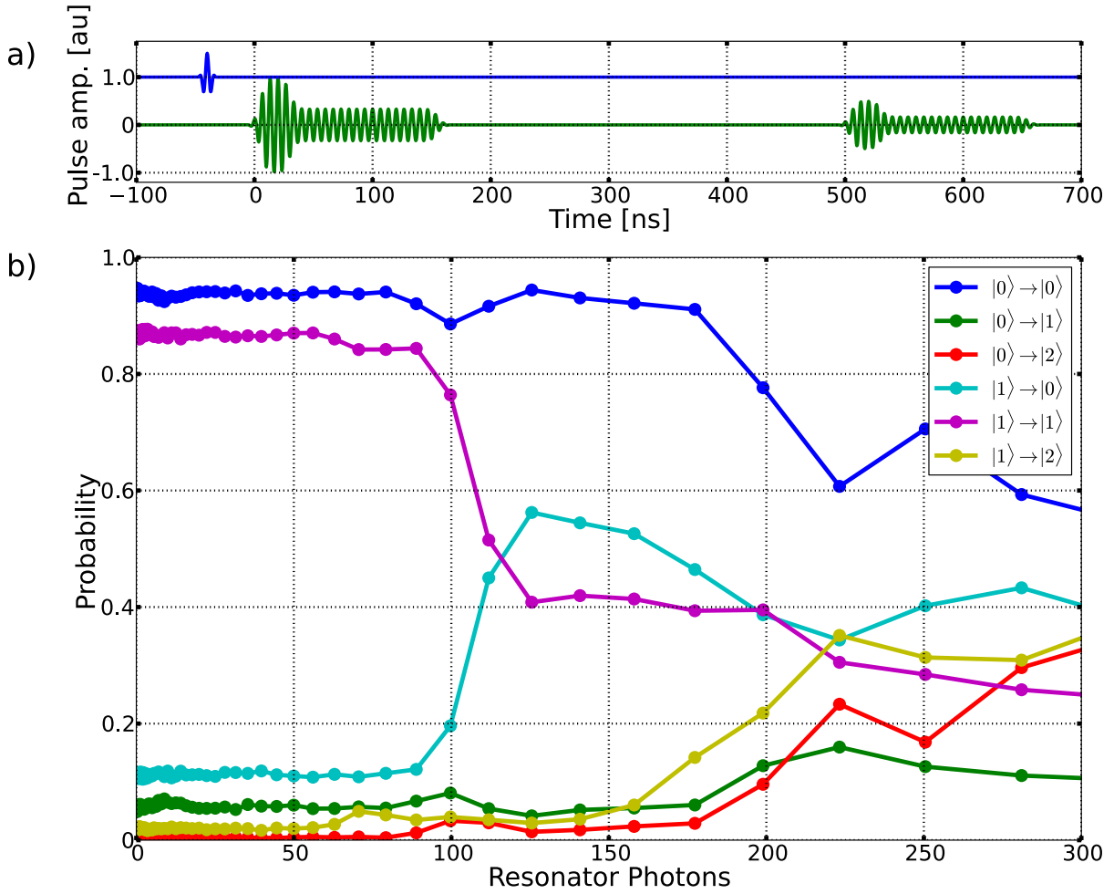
Figure 6.5: Qubit transitions stimulated by the measurement pulse. a) Pulse sequence. The qubit is prepared into the |0\rangle ( |1\rangle ) state with an idle ( \pi -pulse) as shown in blue. We then drive the measurement resonator with a variable power pulse, as shown in green. This pulse can induce qubit state transitions. After a ring-down period, we probe the measurement resonator with a low power pulse to measure the state of the qubit. b) Probabilities for the final state of the qubit for initial states |0\rangle or |1\rangle . Each curve labelled |i\rangle \rightarrow |f\rangle gives the probability that the qubit prepared in state |i\rangle is measured at the end of the sequence to be in state |f\rangle .
