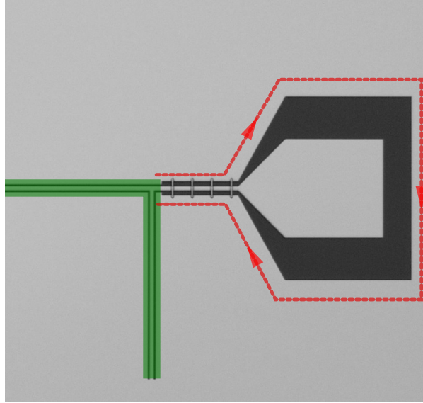
Figure 4.8: Micrograph of the filter tap off point and bond pad. Without crossovers, part of the current return path would flow around the wire bond pad, as shown by the dotted line. The large perimeter of the bond pad would introduce inductance into the return path of filter current and shift the frequency of the filter. Dielectric crossovers connect the ground planes on either side of the tap off path, thus shorting the inductance of the bond pad.
