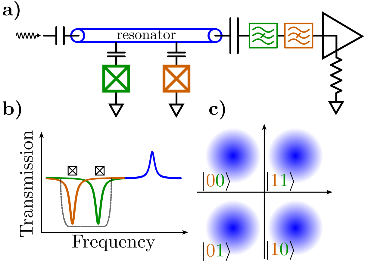
Figure 4.1: Notch filter circuit topology. a) A single resonator (blue) interrupts the microwave feed line in series. Several qubits are coupled in parallel to the single resonator mode. Notch filters (green and brown) on the resonator output protect the qubits against from emission. b) The resonator mode produces a strong transmission peak, while the notch filters produce dips. The qubit frequencies are matched to the filters. c) The qubit states are distinguished in the amplitude-phase plane for the resonator mode.
