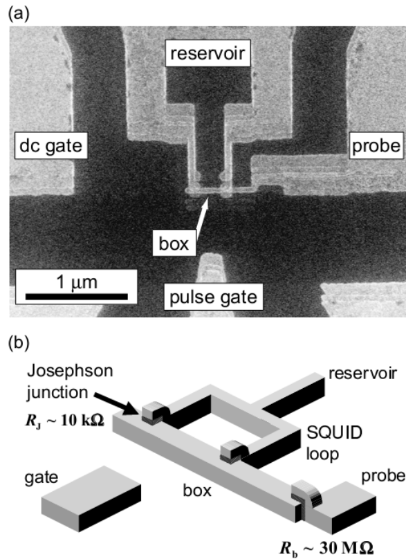
Figure 2.1: The charge qubit used in the first time resolved superconducting qubit measurements. (a) Micro-graph of the device in which can be seen the charge reservoir and superconducting island (“box”). The probe electrode on the right is used for charge based state detection. Note the extremely small scale of the device. This was needed so that the self capacitance energy would be much larger than the junction tunnelling energy, which allows charge to be a well-defined (ie. semiclassical) quantity. (b) Schematic of the device showing the geometry of the reservoir, box, and probe electrodes. The image was taken from Ref. [33].
