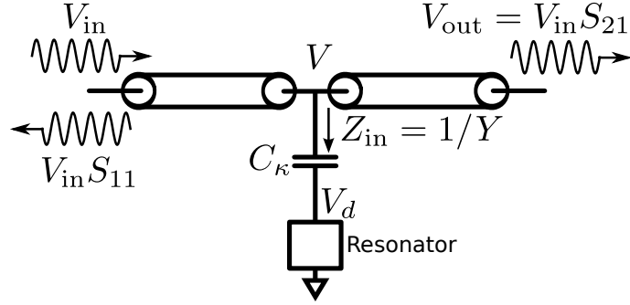
Figure 3.1: A transmission line shunted by a resonant circuit. In incoming voltage wave is partially reflected and partially transmitted by the impedance mismatch at the point where the resonator is coupled to the transmission line.
