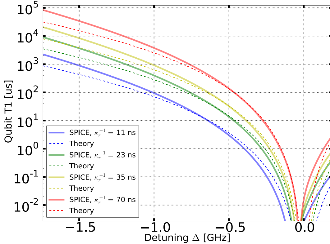
Figure 4.5: Qubit T_1 imposed by the measurement circuit versus qubit-resonator detuning for several values of the resonator decay time. The filter quality factor is Q_F = 30 .
