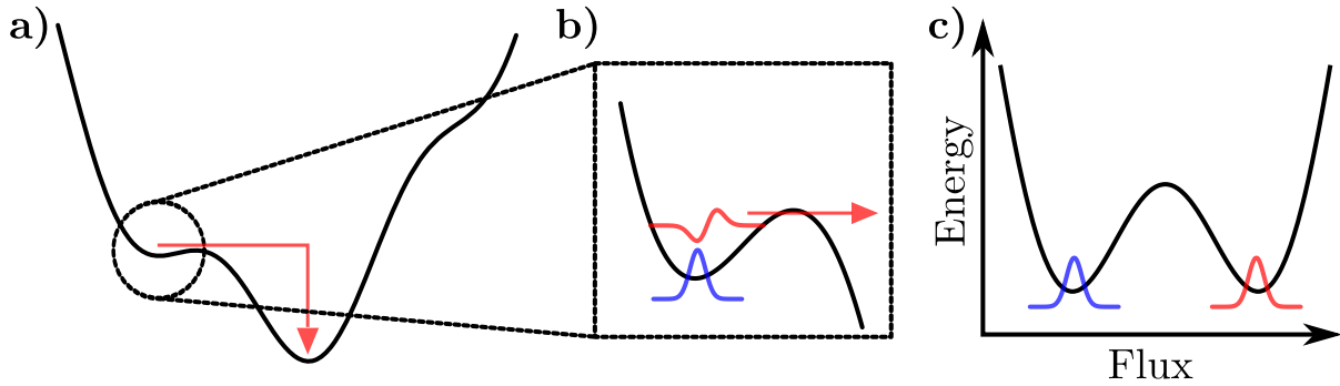
Figure 2.3: The phase qubit. a) The phase qubit is operated such that the wave function sits in an asymmetric shallow well of the potential energy. Tunneling out of this well is used as a mechanism for measurement. b) The ground (blue) and excited (red) states in the shallow well are meta-stable. By momentarily lowering the height of the potential barrier, the excited state tunnels out of the well, while the ground state remains in the well. c) Once the excited state has tunneled, external bias is used to bring the potential into a symmetric shape where the states are separated by a large flux and can be measured with a SQUID.
