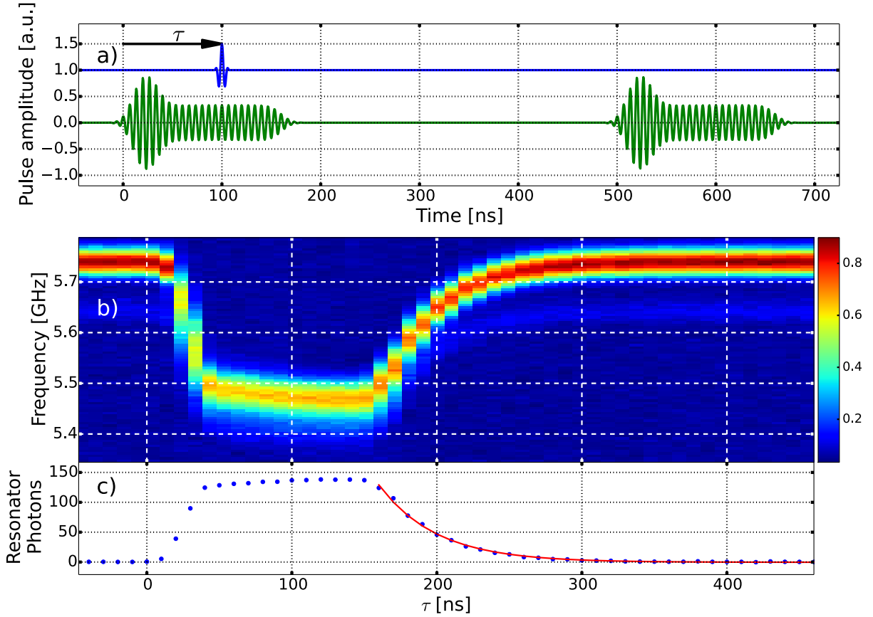
Figure 6.3: Resonator photon occupation during the measurement pulse. a) The control sequence applied to the I port of the IQ mixer used to control the resonator and qubit. We apply two measurement pulses (green) to the resonator. Note the emphasis at the beginning of the pulse which acts to ring up the resonator faster than the ring-up time 1/\kappa_r . During the first pulse, we apply a \pi -pulse (blue) to the qubit at a variable time \tau and frequency. Only when \omega_{\text{probe}} matches the qubit frequency is the qubit excited. The second measurement pulse checks whether or not the qubit was excited by the \pi -pulse. b) Probability (color scale) of qubit excitation versus time and frequency of \pi -pulse. The curve of high qubit probability provides a measure of the qubit frequency as a function of time during the measurement pulse. c) Qubit frequency converted to resonator photon occupation via Eq. (6.2). The red curve is an exponential fit to the decay.
