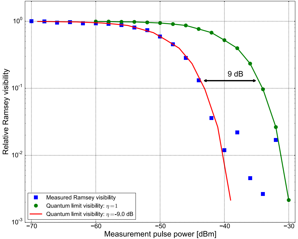
Figure 6.11: Quantum efficiency of the measurement system. Performing a standard Ramsey fringe sequence, but with a measure pulse in between the \pi/2 -pulses, we measure the relative fringe visibility as a function of measure pulse power (blue squares). The fringe visibility data becomes noisy at visibilities < 3\% . We also measure the distinguishability between the qubit states versus measure pulse power, and convert to a quantum limit on Ramsey fringe visibility via Eq. (3.44) (green circles). The comparison between these curves is clarified by re-plotting the quantum limit shifted by 9 dB (red line), which goes through the Ramsey visibility points.
