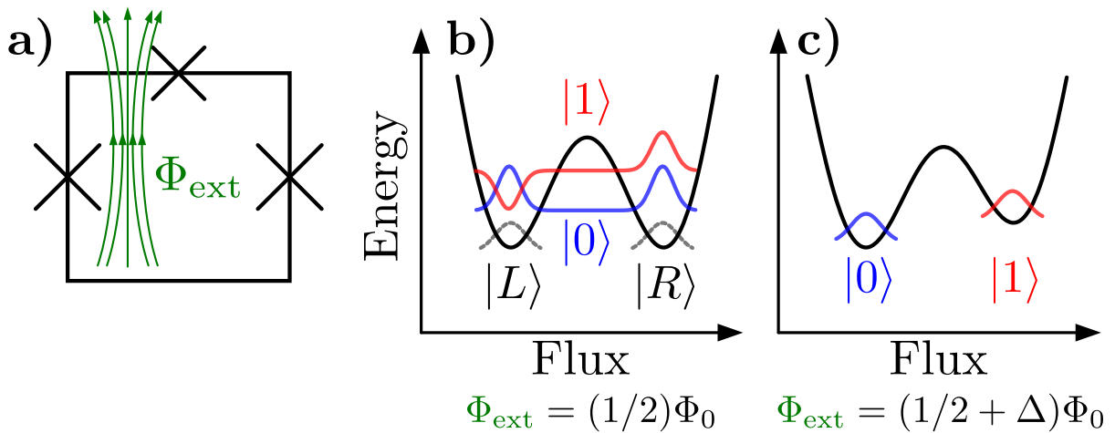
Figure 2.2: Potential energy curves and circuit diagram for the flux qubit. a) The flux qubit is a superconducting loop interrupted by three Josephson junctions, one with lower critical current than the other two. An external bias flux \Phi_{\text{ext}} controls the shape of the energy potential. b) When the system is biased by an external flux of \Phi_0/2 the potential is symmetric. In the absence of quantum tunnelling, there would be two degenerate ground states localized within the potential wells, as shown in gray. Tunnelling causes these states to hybridize into symmetric and anti-symmetric states as shown in blue and red respectively. c) When the external flux bias is changed from \Phi_0/2 (increased or decreased) the degeneracy of the left and right states is removed, and |0\rangle and |1\rangle localize into the left and right wells.
