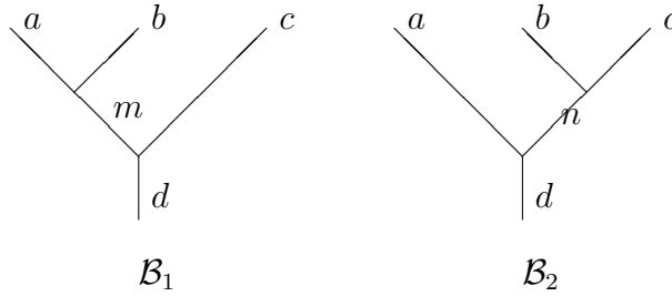
Figure 3.5: Two Bases \mathcal{B}_1 and \mathcal{B}_2
