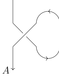
Figure 2.12: The twist \theta_A
