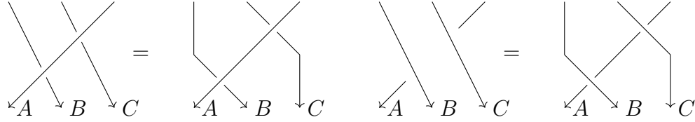
Figure 2.9: Equalities of the braiding
