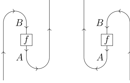
Figure 2.4: f^* (Left) and *f (Right)
