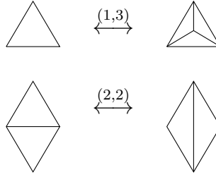
Figure 4.6: Pachner moves (1, 3) , (2, 2) ; n = 2
