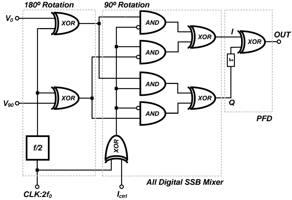
Figure 4.4: The core blocks of the EIC including the Digital-single sideband mixer (D-SSBM) and Quadri-correlator PFD. Courtesy of E. Bloch [1, 2]
