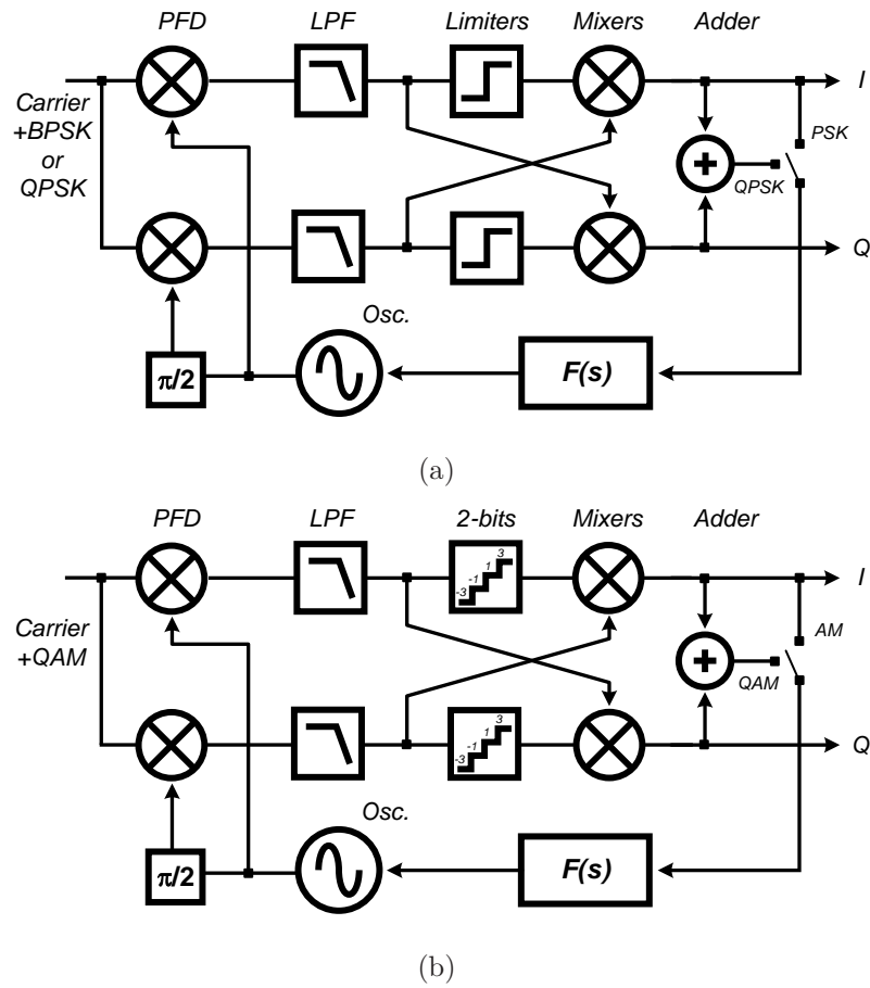
Figure 6.1: Concept schematics for modified Costas loops. QPSK or PSK (a) and QAM or AM (b) [1].
