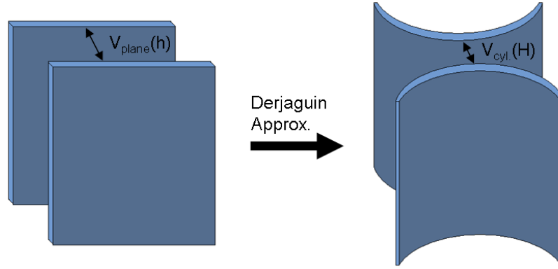
Fig. 3.8| The Derjaguin approximation takes planar potential energies and converts them to equivalent potential energies for curved surfaces. In our particular case, the electrostatic planar potential for surface-to-surface distance h is "bent" to an equivalent potential for two parallel cylindrical surfaces with surface-to-surface distance H
