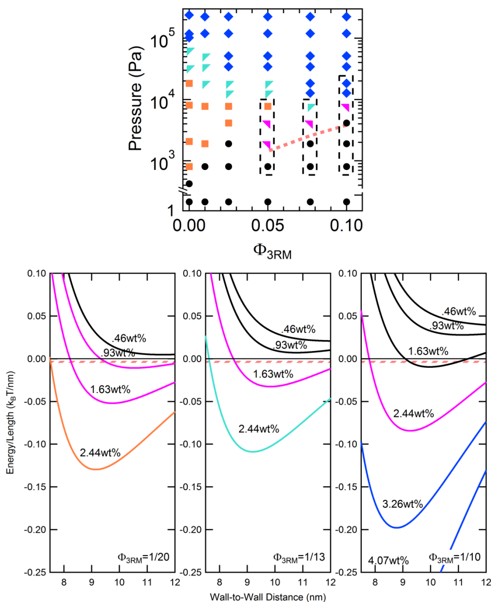
Fig. 3.16| The charged brush model for 3RM Tau at higher coverages of Tau is in closer agreement with experimental behavior. At osmotic pressures taken from selected experimental data points (top), the normalized potential energy per unit length curves were plotted for \Phi_{3RM}=1/20 , 1/13 , 1/10 (bottom), with the color of each model curve corresponding to phase observed experimentally. The phase diagram (top) has been marked (pink-dashed line) at the pressure where bundling is expected, if bundling is assumed to occur at a potential energy depth of 7.5 \text{ k}_B T for 2 \text{ }\mu\text{m} length MTs (see Fig. 3.10). The potential energy curves (bottom) also have a pink-striped zone, which corresponds to a potential energy depth of 5 to 10 \text{ k}_B T .
