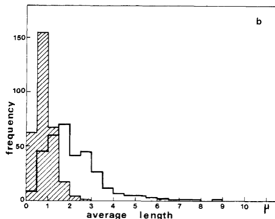
Fig. 3.10| The length distributions for taxol-stabilized microtubules. Near stoichiometric amounts of taxol to tubulin, the average length of microtubules is identified using electron microscopy and plotted after 1 min (hatched bars) and 30 mins (thick bars) 80 . The average length is taken to be 2 \mu\text{m}
