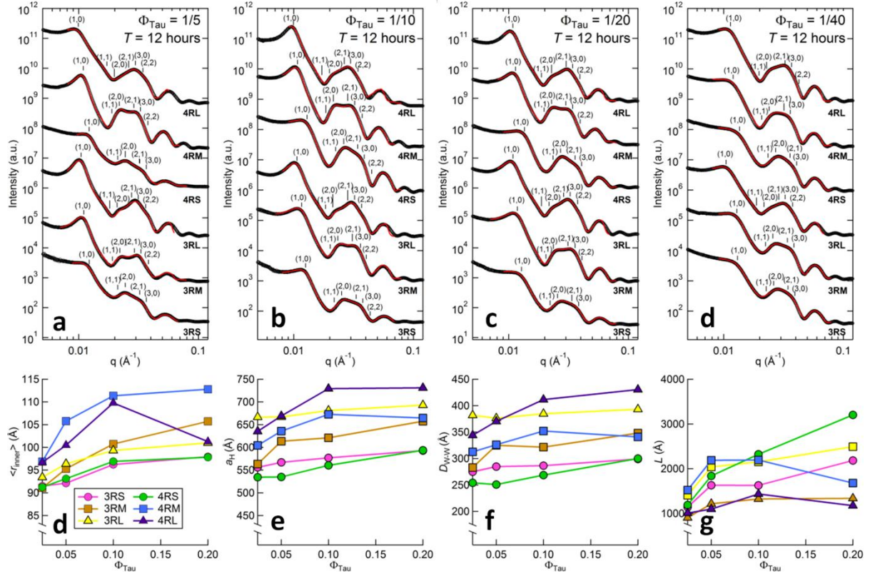
Fig 4.6| Over a physiological range of \Phi_{\text{Tau}} ( 1/40 \geq \Phi_{\text{Tau}} \geq 1/5 ), SAXS and subsequent analysis show the Tau-induced show that microtubule wall-to-wall distance is relatively consistent and is primarily a function of the Tau projection domain length. As before, azimuthally-averaged SAXS data of tubulin mixed with Tau [ \Phi_{\text{Tau}} = 1/5 (a), \Phi_{\text{Tau}} = 1/10 (b), \Phi_{\text{Tau}} = 1/20 (c), and \Phi_{\text{Tau}} = 1/40 (d)] at T = 12 hours with subsequent line-shape analysis [fits in red on data in (a-d)] revealing the ensemble-averaged inner radius \langle r_{\text{in}} \rangle (e), hexagonal lattice parameter a_{\text{H}} (f), wall-to-wall distance D_{\text{w-w}} (g), and bundle domain width L (h). Although D_{\text{w-w}} changes slight as a function of \Phi_{\text{Tau}} , D_{\text{w-w}} is more directly a function of the Tau projection domain length. Generally, increasing Tau concentration also increases the bundle domain width L , in agreement with suppressed microtubule dynamic instability with increasing Tau.
