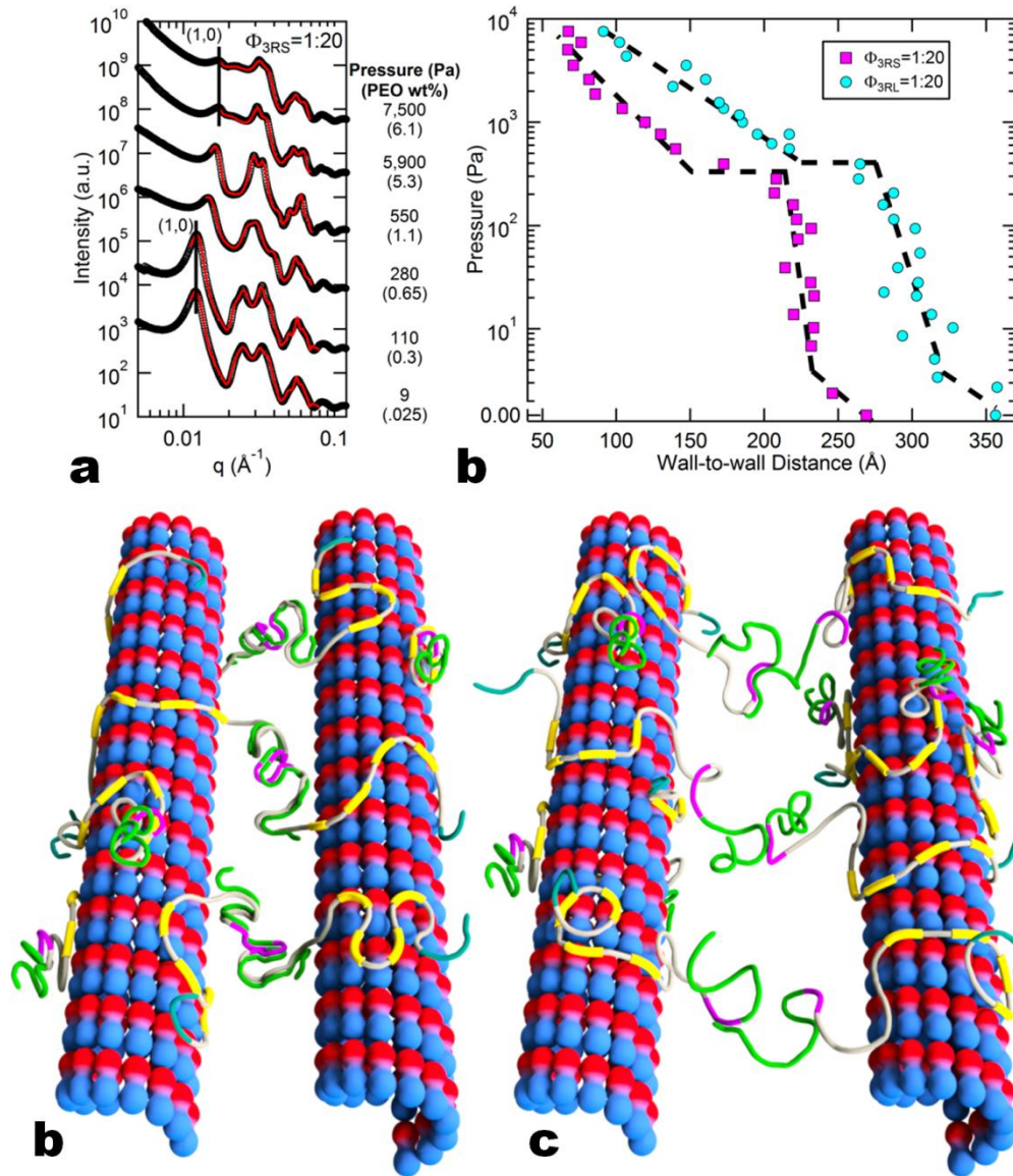
Fig. 4.4 | Direct force measurements of Tau-mediated active microtubule bundles at 37° C in 2 mM GTP reveal distinct energy minima. a , Representative azimuthally-averaged SAXS data for \Phi_{3RS}=1/20 at selected increasing pressures resulting in increasing peak position of q_{10} , reflecting the decrease in the hexagonal lattice parameter a_H . b , The measured wall-to-wall distances ( D_{w-w} ) for 3RS and 3RL mediated microtubule bundles show a sudden transition ( \approx 5 nm decrease) at applied osmotic pressure P \approx 300 -400 Pa, indicative of a secondary energy minimum for microtubule bundles. c , A cartoon of the osmotic-pressure induced secondary minimum at intermediate D_{w-w} , with anti-parallel dimerization occurring between the anionic section of the NTT (green) and the cationic part of the PD (purple) plus cationic proline-rich region (gray). d , A cartoon of the widely-spaced energy minimum, with Tau mediating microtubule bundles by transient charge-charge attractions between the cationic residues (purple/gray) and the anionic residues (green) in the amino-terminal tail.
