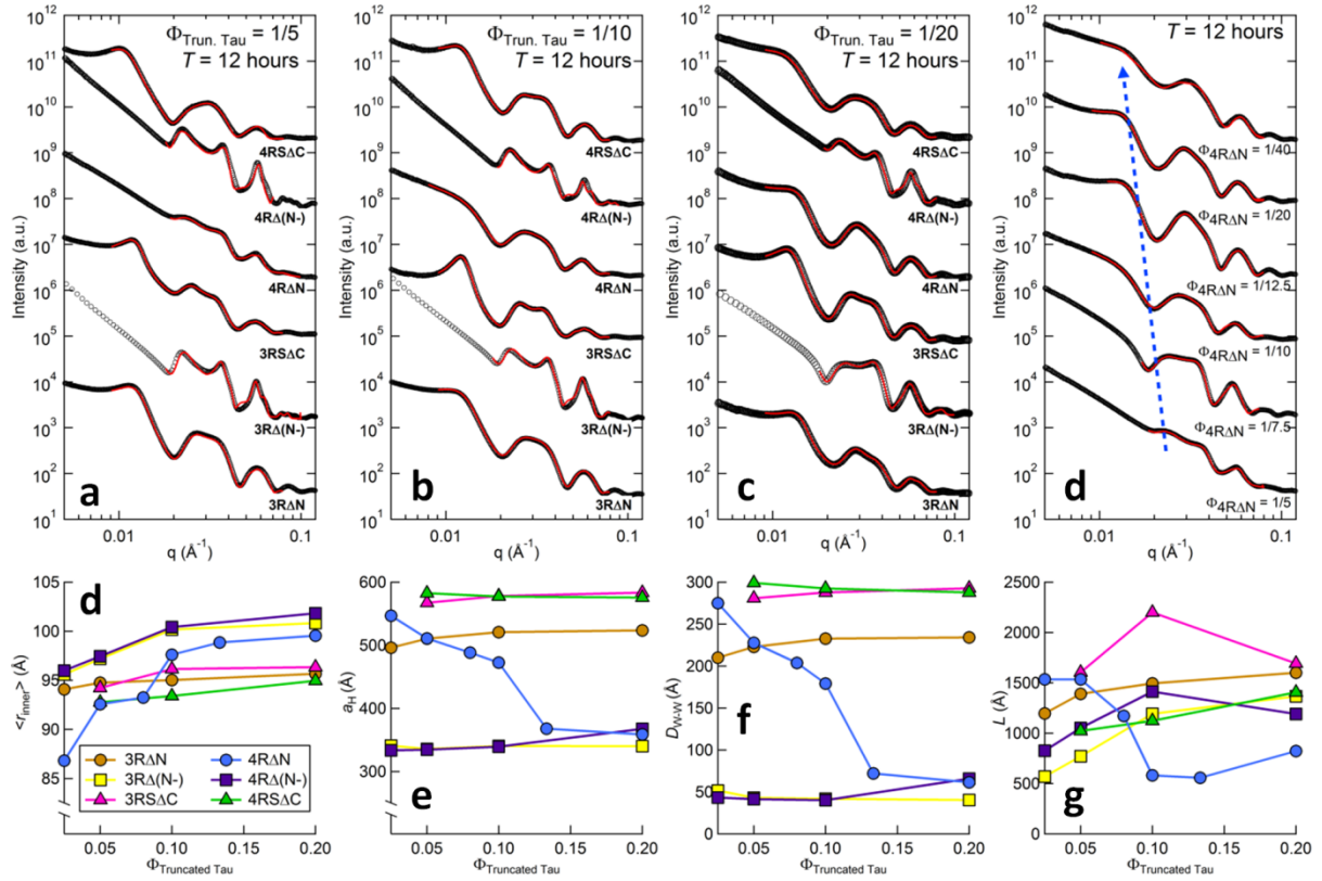
Fig 4.8 | Surprisingly, reaction mixtures with 4R \Delta N Tau (but not 3R \Delta N) undergo a phase transition from widely-spaced to tightly-packed microtubule bundles with increasing truncated Tau concentration. As before, azimuthally-averaged SAXS data of tubulin mixed with truncated Tau [ \Phi_{\text{Trun. Tau}} = 1/5 (a), \Phi_{\text{Trun. Tau}} = 1/10 (b), and \Phi_{\text{Trun. Tau}} = 1/20 (c)] reveal hexagonally-ordered bundles, albeit with varying morphologies. Dramatically changing line profiles for reaction mixtures with 4R \Delta N prompted higher resolution investigation a function of Tau concentration [ \Phi_{\text{Trun. Tau}} = 1/5 , 1/7.5 , 1/10 , 1/12.5 , 1/20 , and 1/40 (d)] with phase transition observed from widely-spaced to tightly-packed bundles for increasing 4R \Delta N concentration. Line-shape analysis [subsequent fits in red on data in (a-d)] reveals the ensemble-averaged inner radius \langle r_{\text{in}} \rangle (e), hexagonal lattice parameter a_H (f), wall-to-wall distance D_{\text{w-w}} (g), and bundle domain width L (h), with clear transition observed in (f) and (g).
