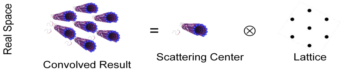
Figure 2.5 | A system of scattering centers in a lattice can be mathematically described as the convolution ( \otimes ) of the scattering center with the lattice.
