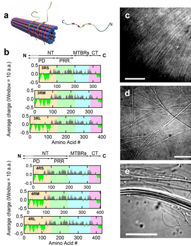
Fig. 3.1| MAP Tau binds to the microtubule surface and modulates the higher-order structure of microtubules with increasing osmotic pressure. (a) Schematic of a microtubule with bound Tau protein (left) and a single Tau protein (right, labeled with N- and C- terminus ends) with four MT-binding repeats (colored boxes). (b) Charge (averaged over 10 residues) versus amino acid residue number for six isoforms of human Tau. The charge distribution diagram of each isoform shows the cationic (grey) nature of Tau with the exception the amino- and carboxyl- terminal tails which include anionic (bright green) regions, which lead to dipole-like characteristics. The N-terminal (NT) is made up of the projection domain (PD, yellow background, first 92, 121, and 150 AAs for -S, -M and -L isoforms) and proline-rich region (PRR, green background, next 94 AAs), followed by MT-binding region (MTBR, blue background), and ending at the carboxyl-terminus (C) with the C-terminal (CT, pink background). Tau isoforms have either 3 or 4 microtubule-binding repeats (3R-, 4R-) as a result of excluding
