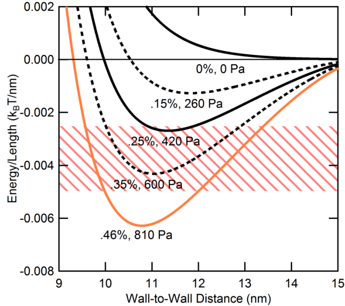
Fig. 3.13| The energy per unit length curves against the wall-to-wall distance utilizing the soft-cylinder model. Curves derived from the model (Eq. 3.16) are plotted for actual PEO wt% used in experiments (solid lines) and in-between concentrations (dashed lines). Colors (from black to orange) are coordinated with data in fig. 3.3 ( \Phi_{\text{Tau}}=0 ). If the bundled state corresponds to a potential energy depth of 5 to 10 k_B T (the pink-striped zone) for 2 \mu\text{m} length MTs (see Fig. 3.10), the model predicts bundling would occur at .46 and .35 wt% of 20k PEO, which is experimentally recapitulated (orange curve).
