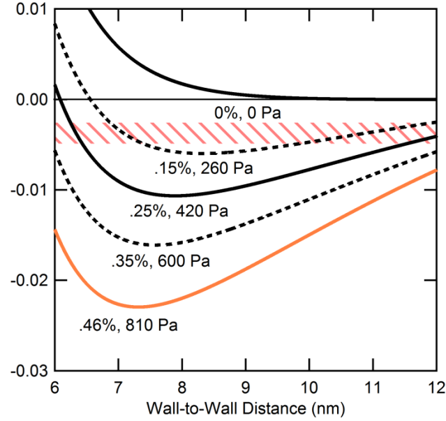
Fig. 3.9| The energy per unit length curves against the wall-to-wall distance using the simple charged-cylinder model for MTs. Curves derived from the model (equation S1.10) are plotted for actual PEO wt% used in experiments (solid lines) and in-between concentrations (dashed lines). Colors (from black to orange) are coordinated with data in fig. 3 ( \Phi_{Tau}=0 ). If the bundled state corresponds to a potential energy depth of 5 to 10 k_B T (the pink-striped zone) for 2 \mu m length MTs (see Fig. 3.10), the model predicts bundling would occur at .15 wt% of 20k PEO (and above) while experimentally bundling is seen between 0.25 and 0.46 wt% of 20k PEO (orange curve).
