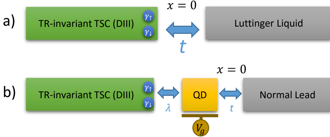
Figure 4.1: Schematic setup consisting of a) a junction between a LL and a TRI topological superconductor, and b) a QD coupled to a NL and a TRI topological superconductor. Here, x = 0 denotes the point in the lead which couples to the MKP or QD.
