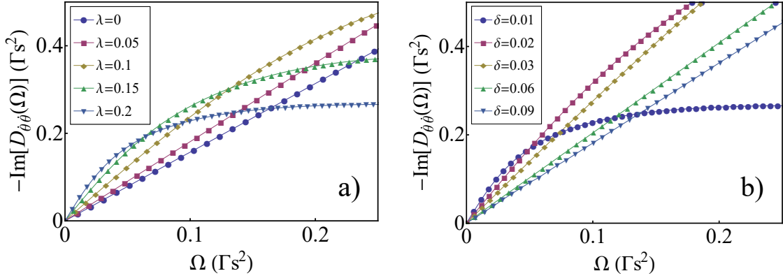
Figure 4.6: The function \text{Im}[D_{\dot{\theta}\dot{\theta}}(\Omega)] for different values of \lambda and \delta . Here panels a) and b) correspond to \delta = 0.01 and \lambda = 0.2 ; we used \Gamma = 1 , \epsilon = -5 , \Lambda = 50 here.
