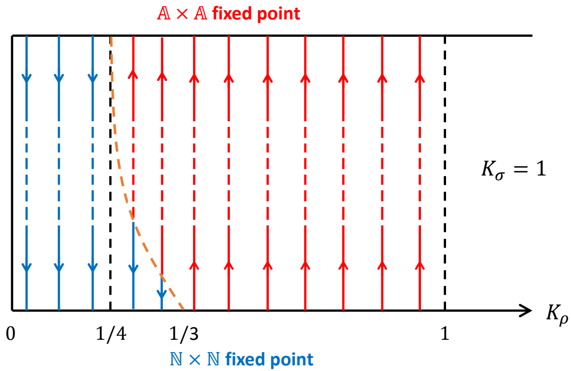
Figure 4.3: Illustration of the flow between the normal reflection fixed point \mathbb{N} \times \mathbb{N} and the Andreev reflection fixed point \mathbb{A} \times \mathbb{A} for the junction with \mathbb{U}(1) spin-rotation symmetry.
