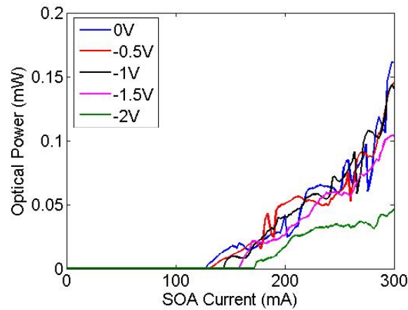
Figure 2.3. Fiber coupled light vs. current curves for counterclockwise (CCW) lasing direction. CCW is with respect to schematic in Figure 2.2 [23] © 2014 IEEE.
