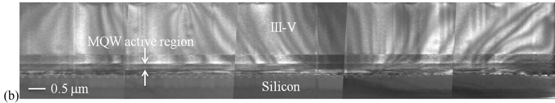
Figure 4.6. (a) Close-up TEM image of a failed device made using an epitaxial wafer with structure A showing no defects in the active layer. (b) A stitched image of a 15 μm long longitudinal cross-section of the same laser diode with no defects in the active layer [62] © 2013 IEEE.
