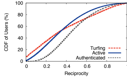
Figure 3.25: Reciprocity.
