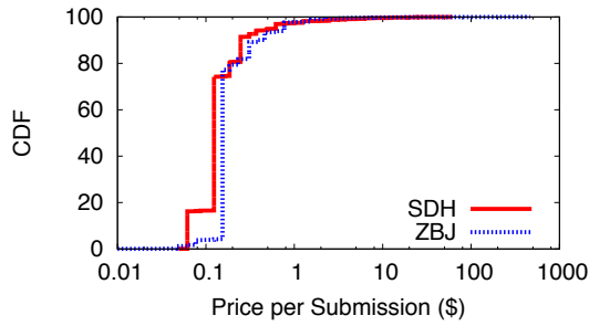
Figure 3.9: Submission prices.
