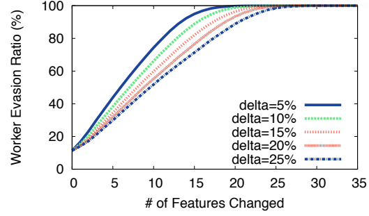
Figure 3.38: Impact of median value estimation error on evasion rate, using DD evasion on SVMp.
