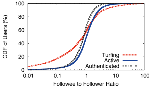
Figure 3.24: Followee-to-Follower ratio.
